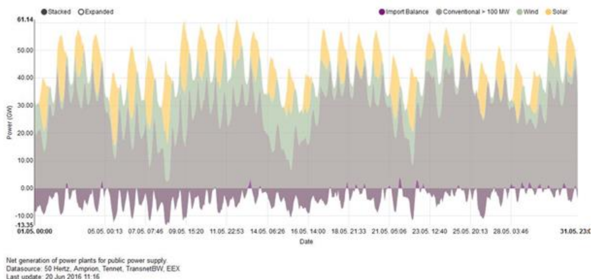
Figure 35: PV (yellow), wind (green), conventional (light grey) power (>100 MW) generation in, and power exports (dark grey) from, Germany in May 2016, Source: (Fraunhofer ISE, 2016)
