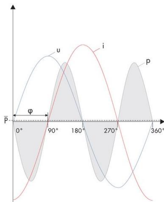
Figure 58: Current and voltage are oscillating with an off- set of 90°; Source: (SMA Solar Technology AG)
