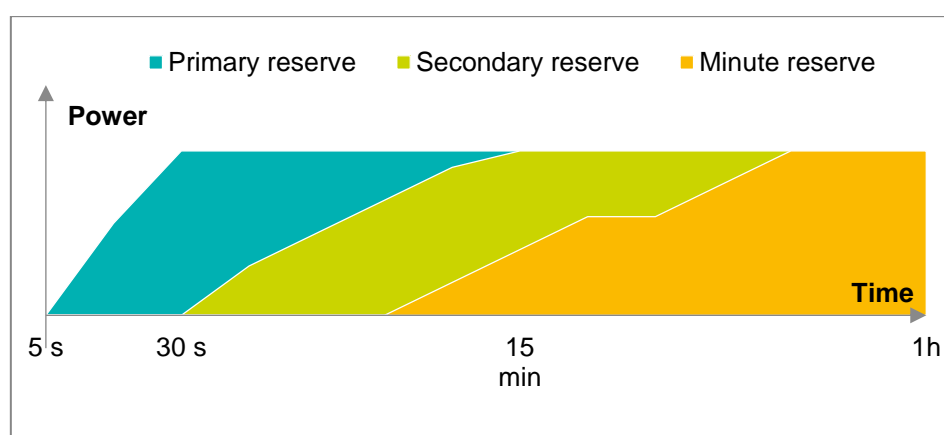
Figure 53: Illustration of the different categories of operating reserve Germany, Source: (B.A.U.M. Consult GmbH, 2014)
