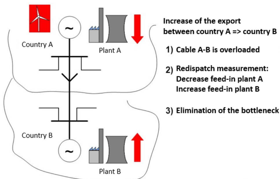
Figure 54: Example redispatch concerning unexpected wind power feed-in, Source: (Fraunhofer IWES, 2014)
