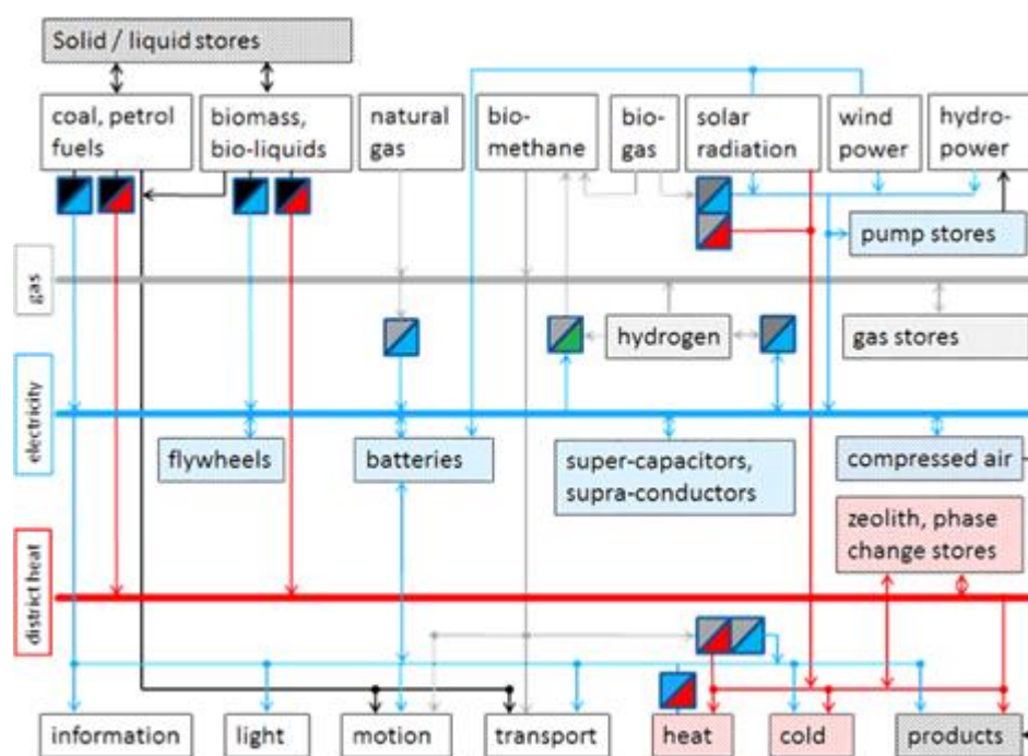
Figure 38: Energy pathways with energy storage, Source: (Stöhr, 2013)
