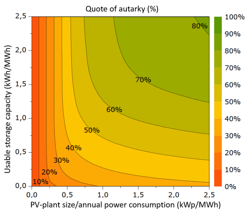
Figure 66: Dimensioning of energetic systems for Germany, Source: (HTW-Berlin, 2013)
