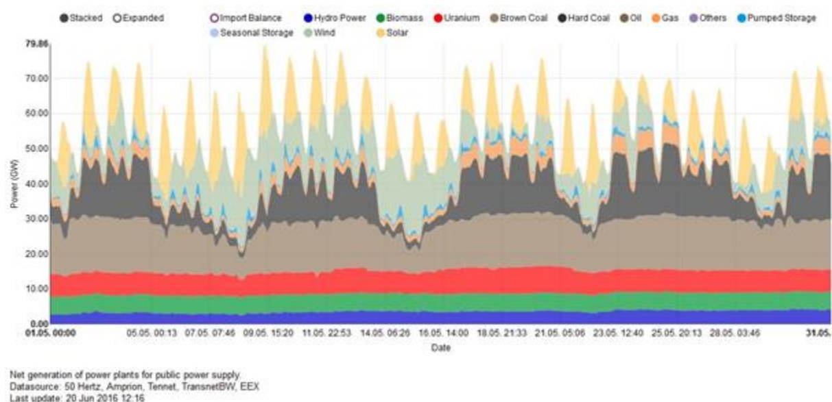
Figure 36: Power generation mix in Germany in May 2016, Source: (Fraunhofer ISE, 2016)
