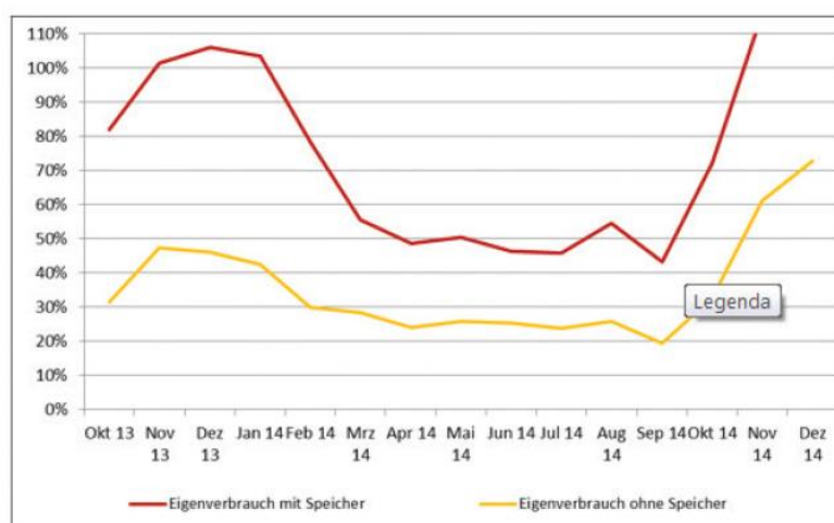
Figure 64: Quote of self-consumption increasing by using a battery storage system, Source: (eza!, 2015)
