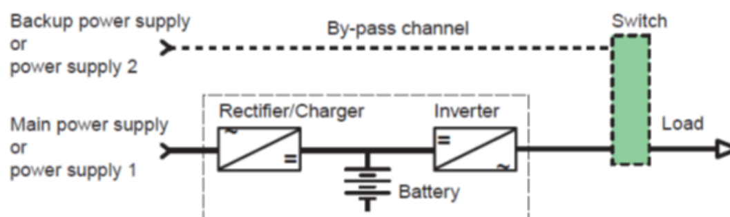
Figure 61: Schematic diagram of a double conversion or online UPS, Source: (Cahier technique n°129 Schneider Electric, 2004)
