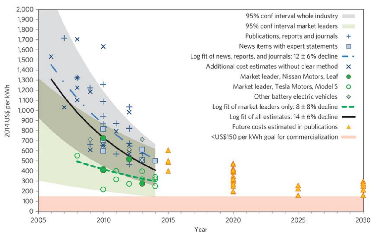
Figure 77: Cost of lithium-ion battery packs; Source: (Nykqvist, et al., 2015)
