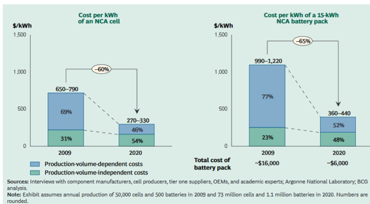
Figure 75: Decline of the battery costs from 2009 to 2020; Source: (Dinger, et al., 2010)
