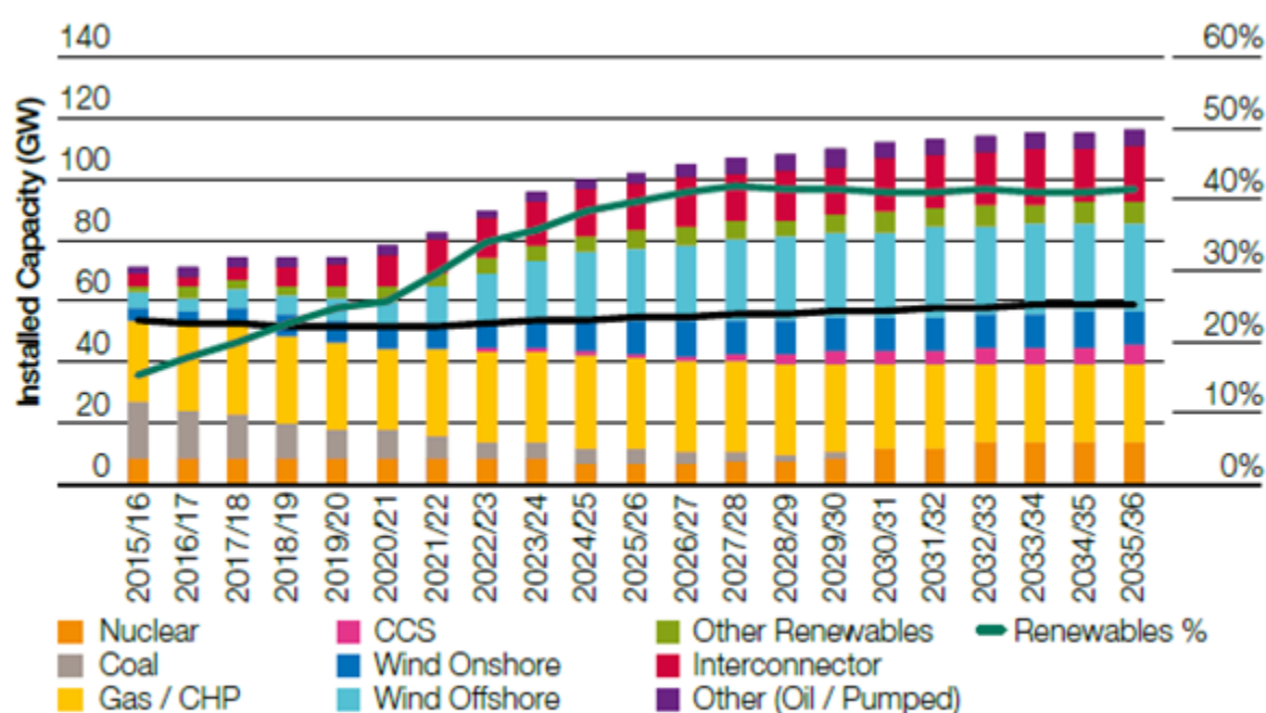
Figure 52: Gone green scenario, Future Energy Scenarios 2015, National Grid (National Grid, 2015).
