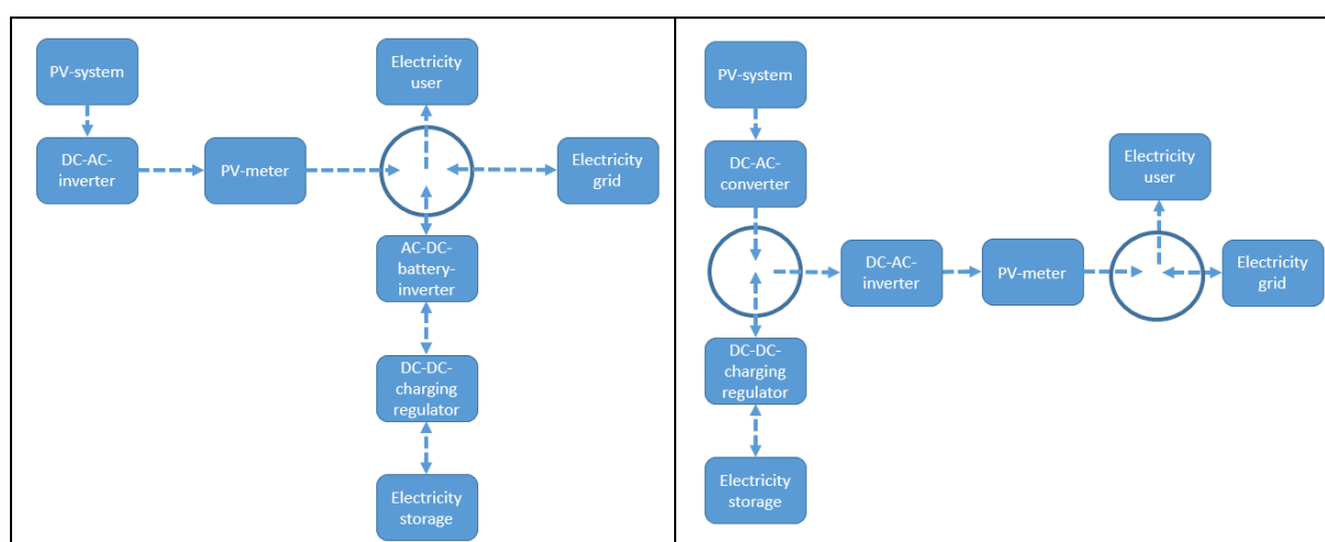
Figure 79: AC- and DC-coupling of an energy storage; Source: (Energie-Experten, 2016)
