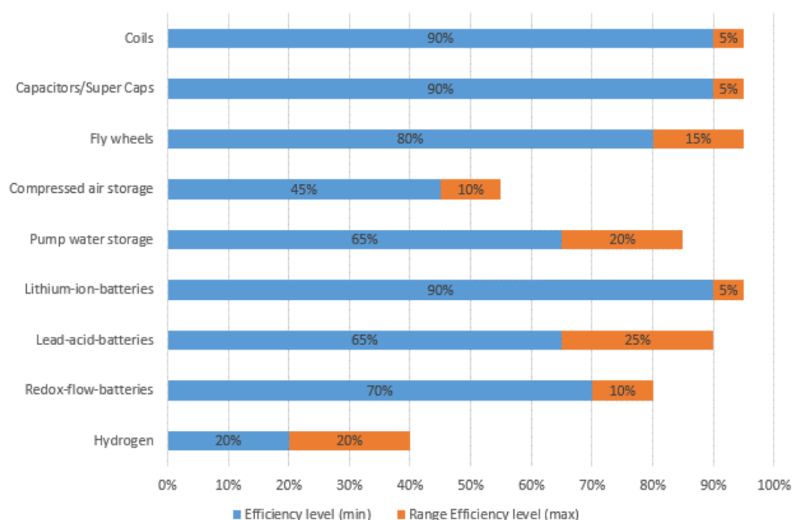
Figure 78: Efficiency level (in percent) of different energy storage systems 2012; Source: (Statista, 2016)
