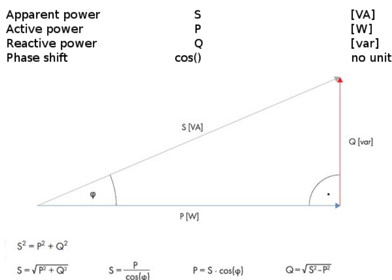
Figure 59: Mathematical relationships between apparent, active and reactive power; Source: (SMA Solar Technology AG)
