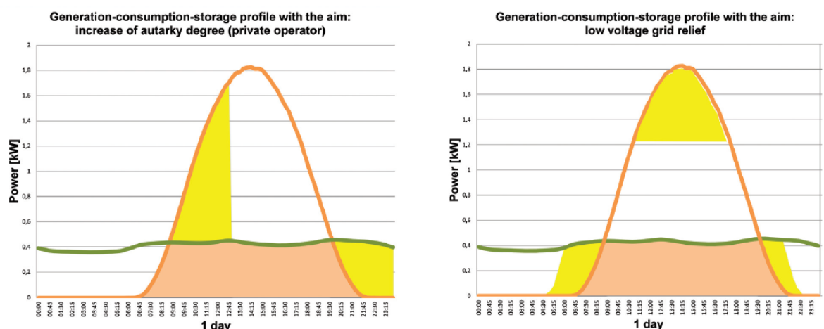
Figure 63: Different generation-consumption-storage profiles, Source: (AÜW, 2015)
