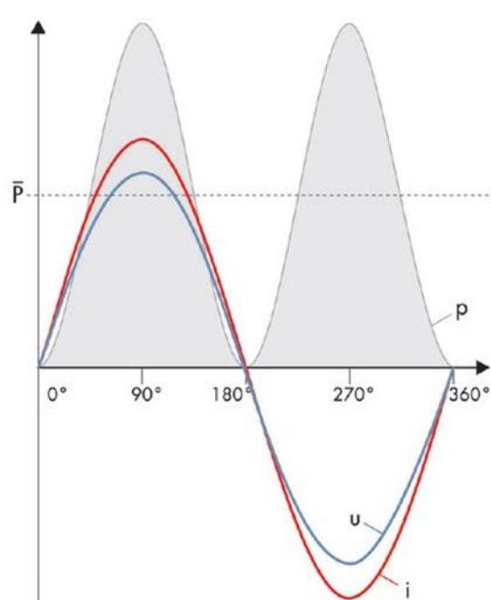
Figure 57: Current and voltage are oscillating Simultaneous; Source: (SMA Solar Technology AG)
