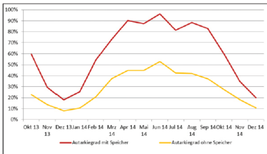
Figure 67: Quote of autarky increasing by using a battery storage system, Source: (eza!, 2015)
